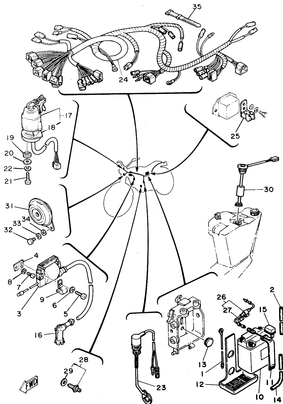
FIG. 34 ELECTRICAL 1
